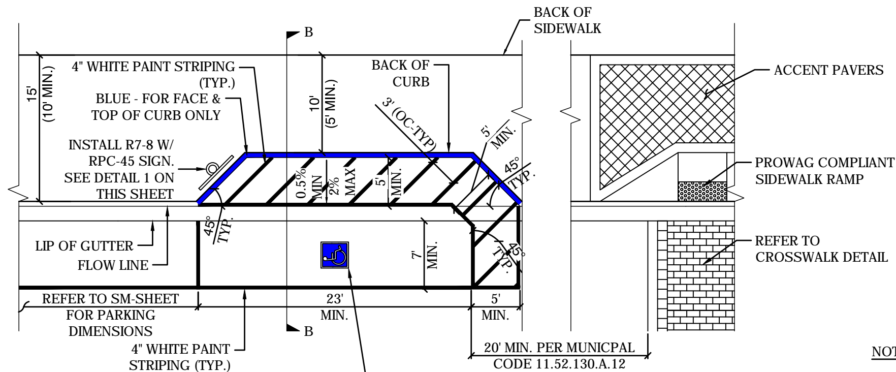
ACCESSIBLE SIGN (MUTCD R7-8 W/ ADD'L LETTERING AS SHOWN)
