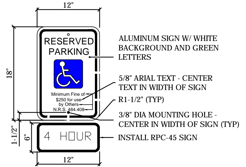
ACCESSIBLE SIGN (MUTCD R7-8 W/ ADD'L LETTERING AS SHOWN)
