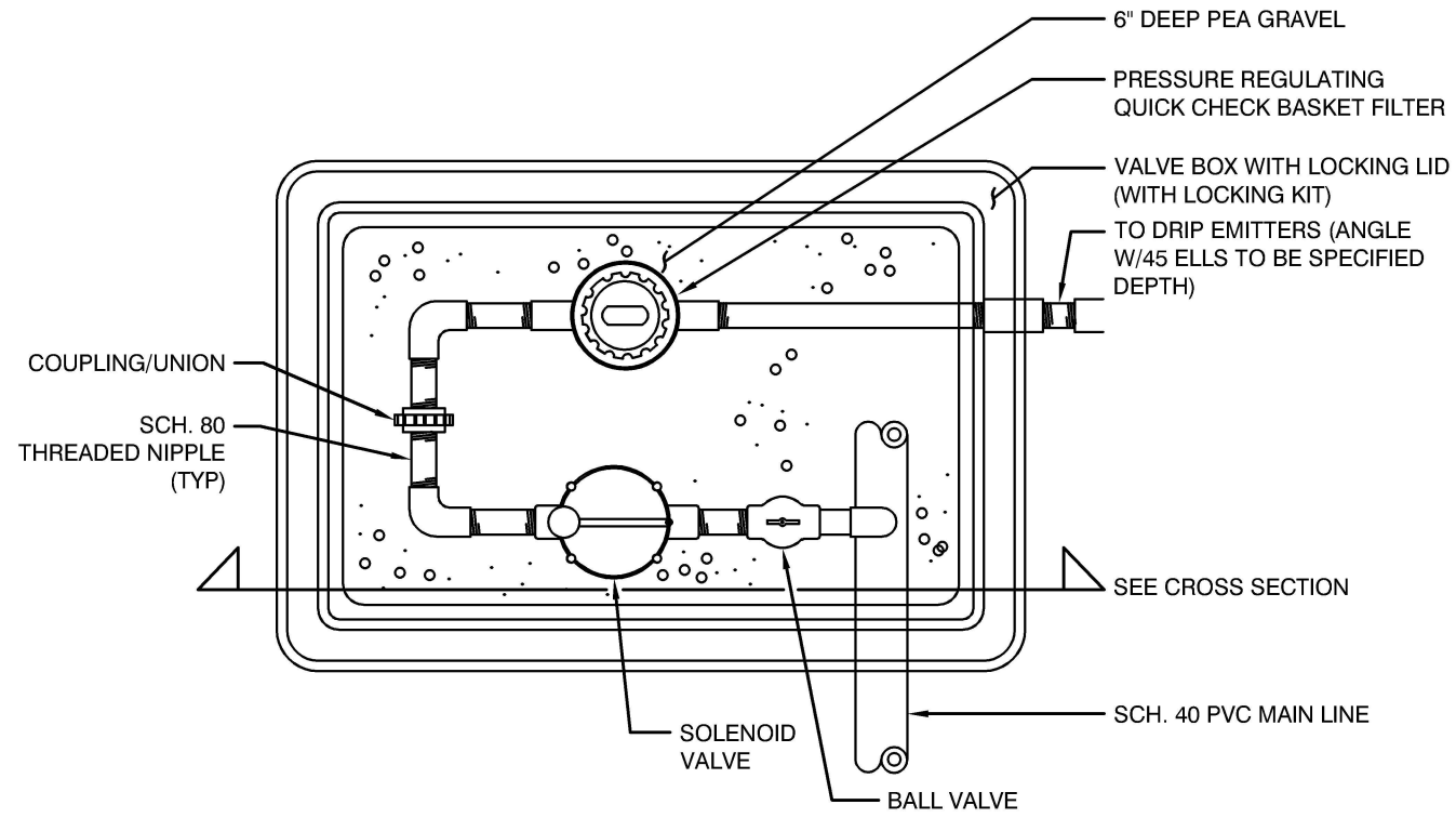
PLAN VIEW
